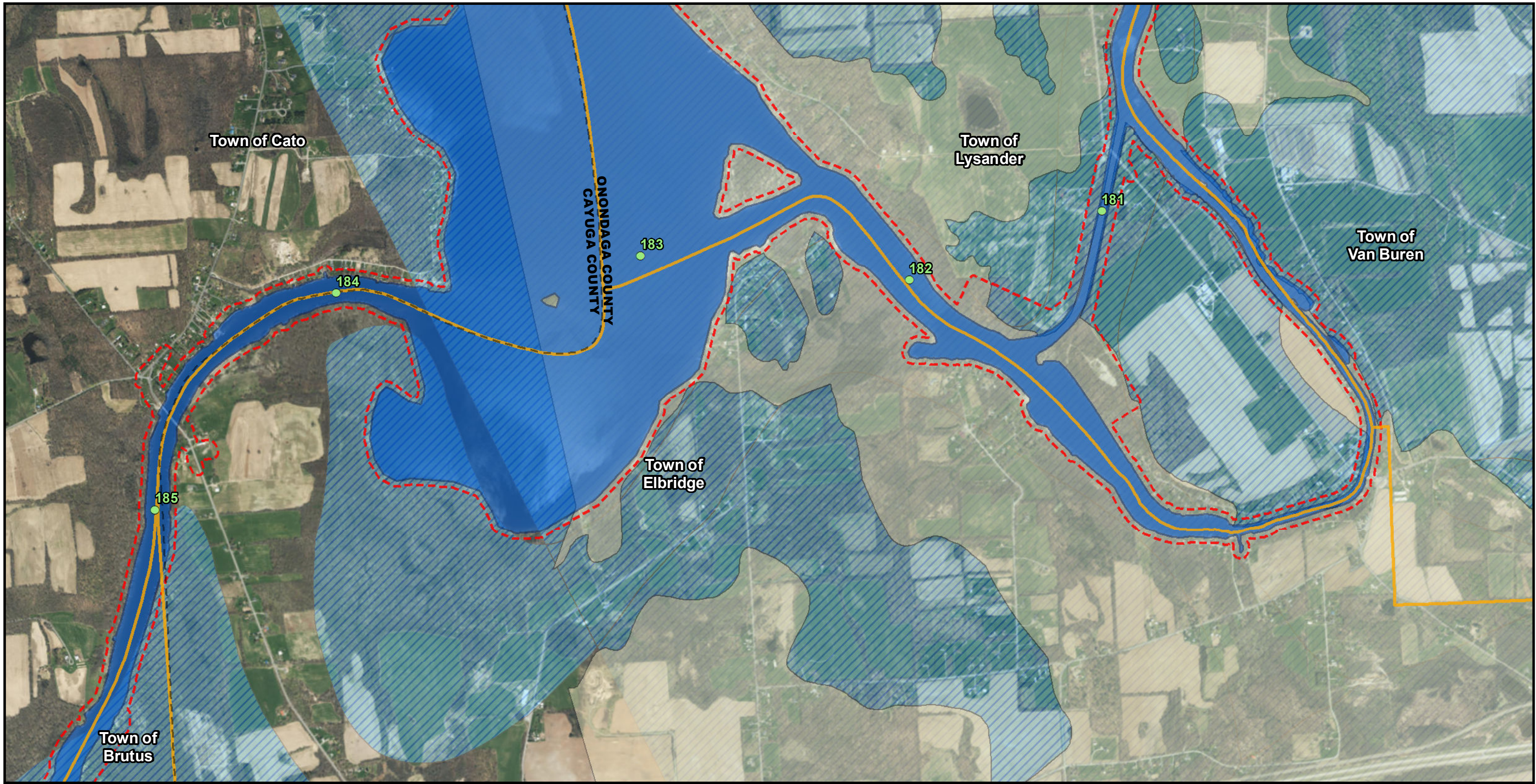
Figure 79F: Aquifers
